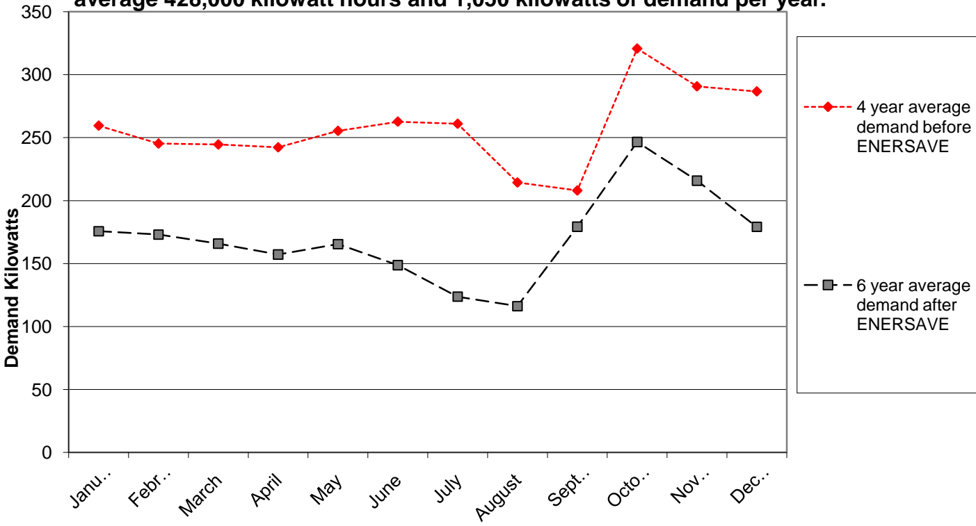
270,000 bushel storage w/pack line. ENERSAVE upgrade saves an average 428,000 kilowatt hours and 1,050 kilowatts of demand per year.
